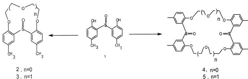
FIGURE 1 Benzosulfoxide macrocycles 2–5.
